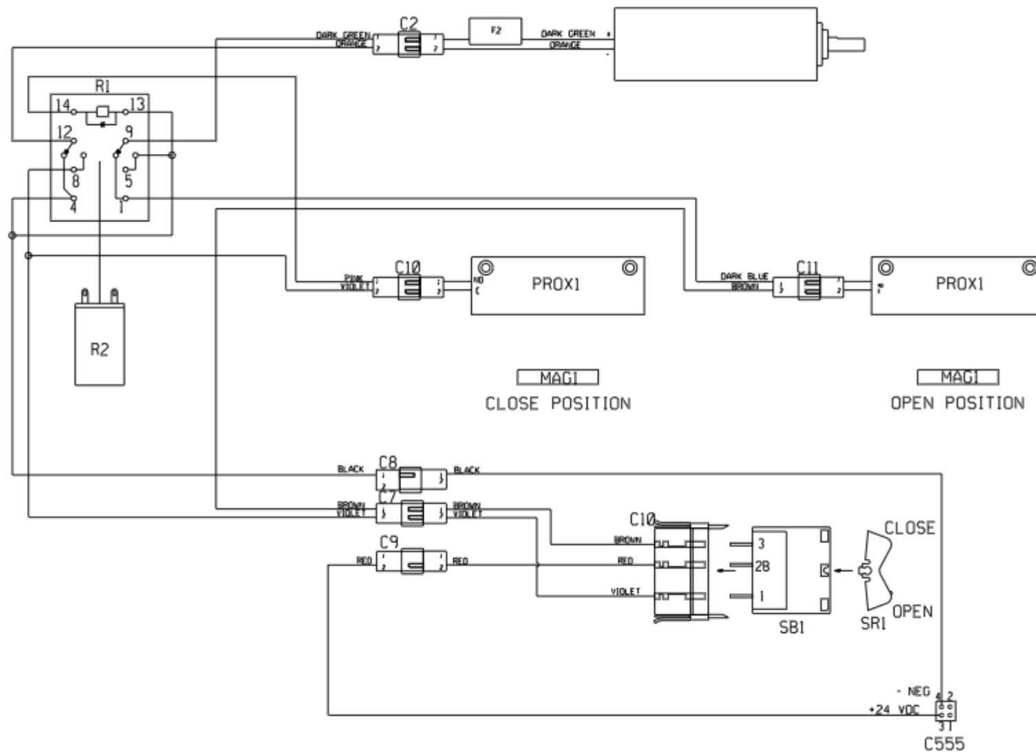
INTERNAL SCHEMATIC SLIDING WINDOW
